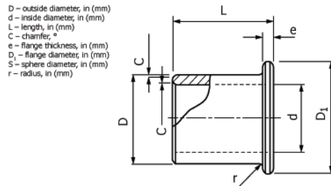
FIG. 2 Standard Flange Bearing
