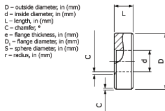
FIG. 3 Standard Thrust Bearing
