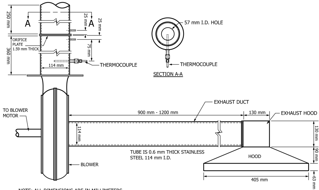
FIG. 3 Exhaust System
