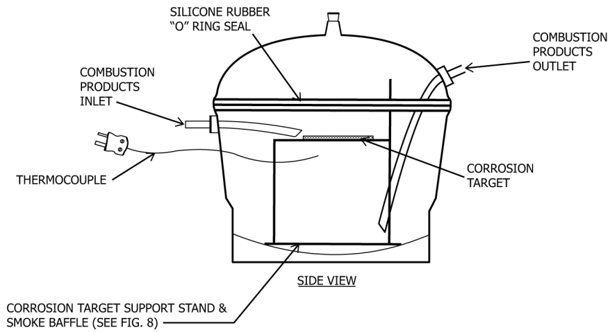
FIG. 10 Exposure Chamber
