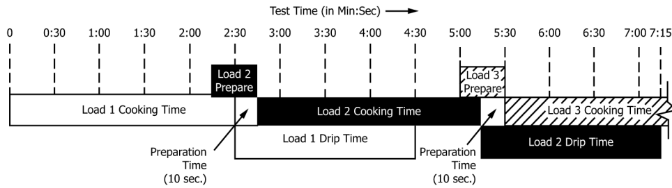
FIG. 1 Sequence of Stir-Up Cook Test (Not to Scale)
