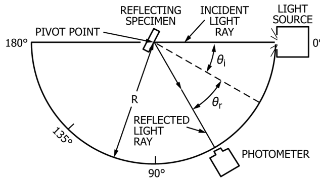
FIG. 1 Apparatus Set-Up
