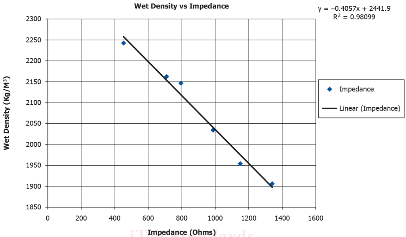
FIG. 3 Typical Values of Wet Density Vs. Impedance (Regression Equation Upper Right) The data points are electrical measured values (X axis) that are used to derive the Wet Density (Y axis).
