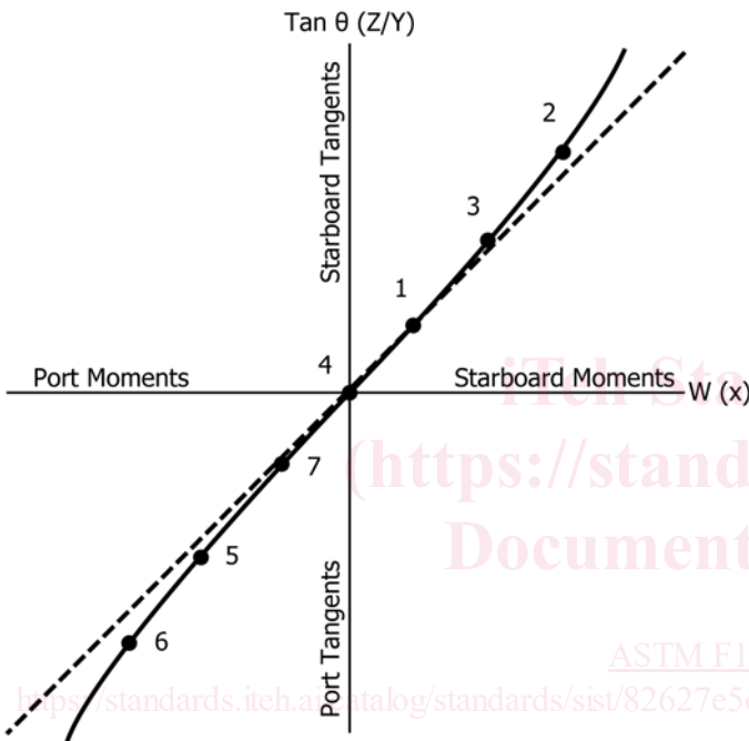
FIG. 5 Measuring the Angle of Inclination
