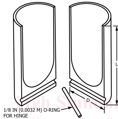
b - MACHINED FIG. 1 Sabot Configuration
