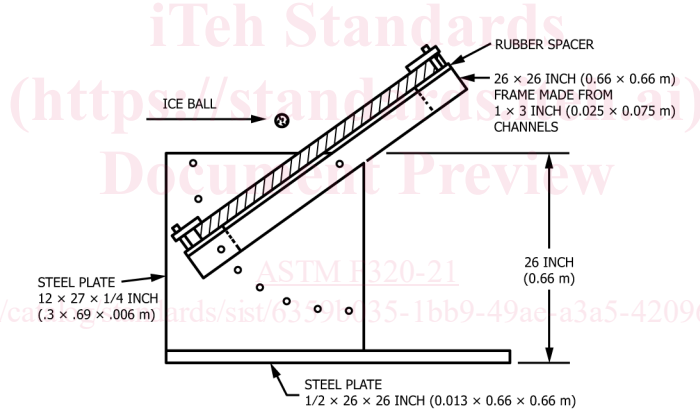
FIG. 7 Example Test Specimen Holder
