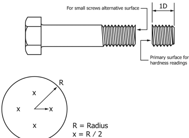
FIG. 1 Hardness Arbitration Test Location
