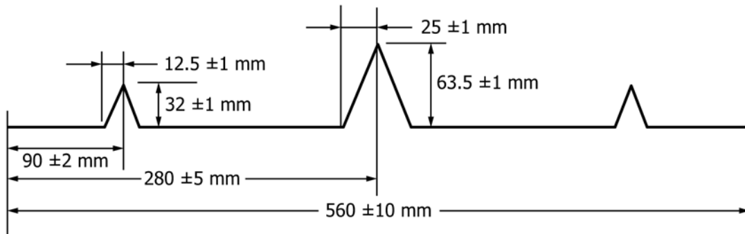
FIG. 1 Specimen and Stress Riser Geometry (4, 3)
