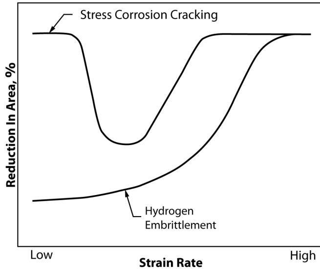
FIG. 2 Schematic of Strain Rate Range
