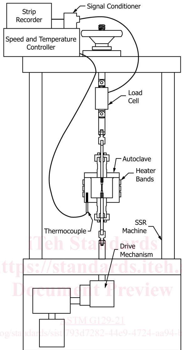
FIG. 1 An Example of a-SSR Testing Machine-Machine
