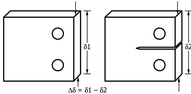
FIG. 1 Residual Stress Correction Practice Distortion Characterization for K_{Ic} Testing of C(T) Specimens
