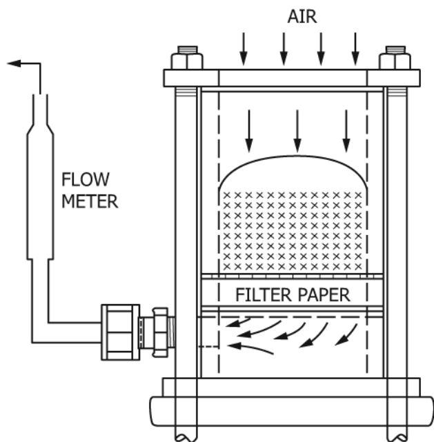
FIG. 3 Apparatus Air Flow Configuration
