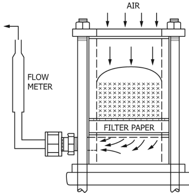
FIG. 3 Apparatus Air Flow Configuration
