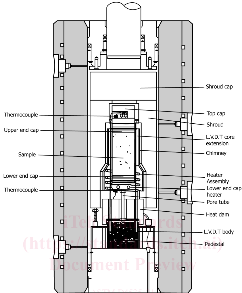
https://standards.iteh.ai/catalog/standards/sist/c1-4678-b302-b89e82c9d01f/astm-d4535-21 Thermal expansion test configuration
