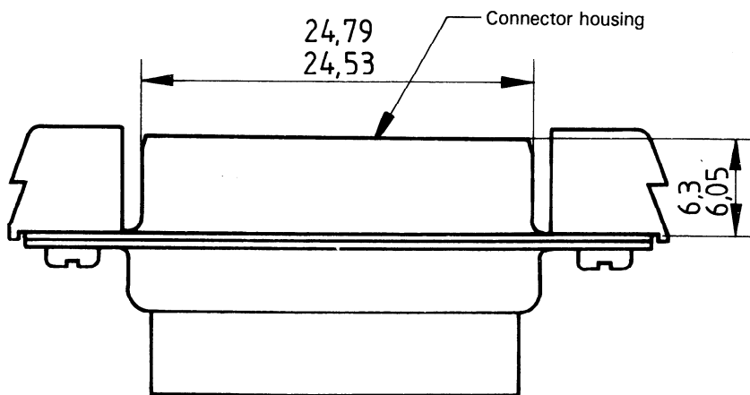
Figure 2 – DCE connector
