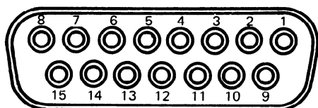
DCE contact arrangement viewed from connector front (DTE side)
