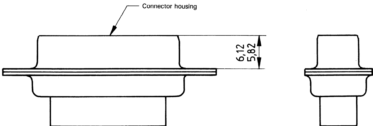
Figure 1 – DTE connector
