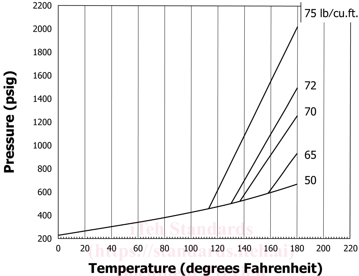
FIG. 2 Isometric Diagram HFC-227ea Pressurized to 360 psig (25.8 bar) With Nitrogen at 70°F (21°C) 70 °F (21 °C)
