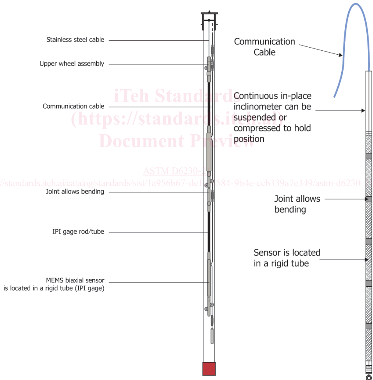
FIG. 2 Typical Components of Method B Inclinometer Systems
