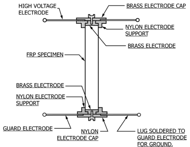
FIG. 5 Assembly Detail
