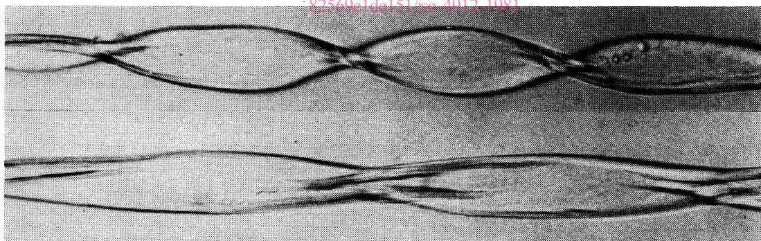
Figure 8 — Immature fibre (type A)
