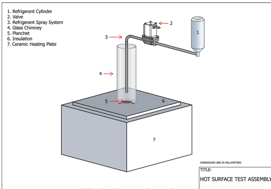
FIG. 1 Hot Surface Ignition Temperature Test Apparatus
