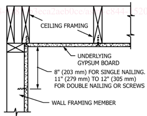
FIG. 4 Vertical Section, Ceiling Framing Parallel to Wall
