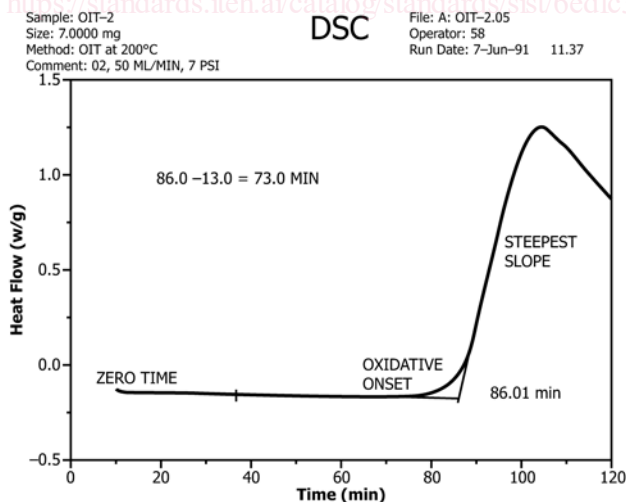
FIG. 3 Determination of OIT
