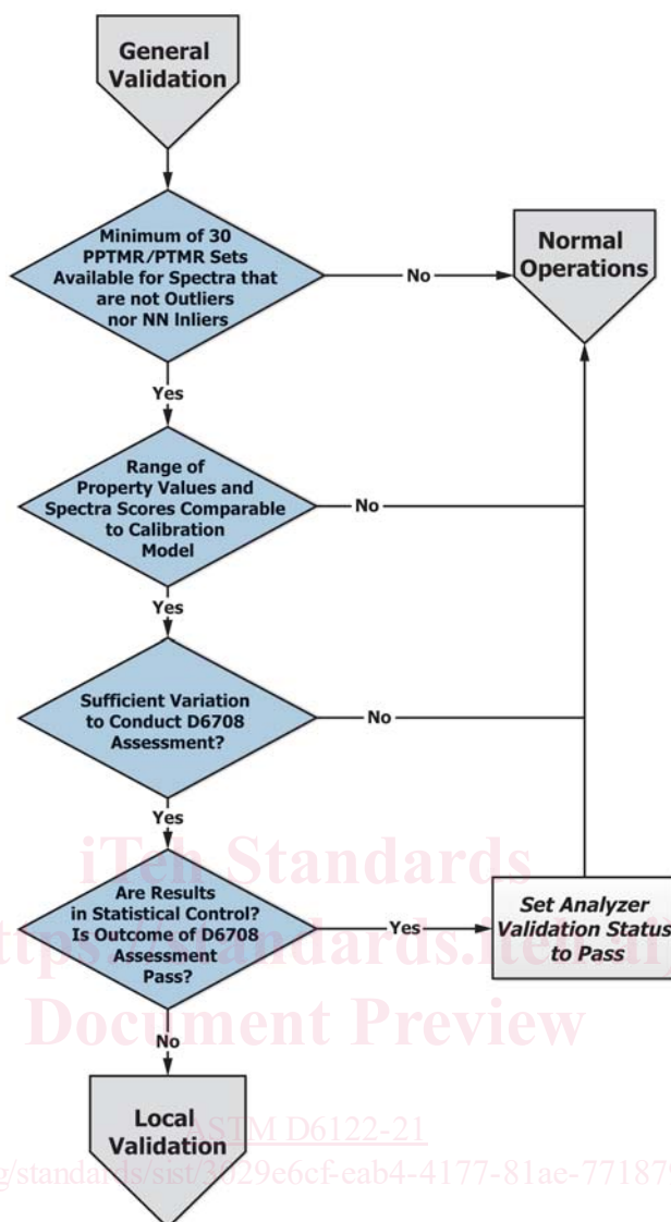
FIG. 6 Flowchart of Process Analyzer Validation Practice General Validation
