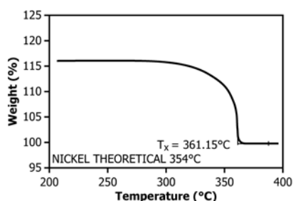
FIG. 1 Magnetic Reference Temperature
