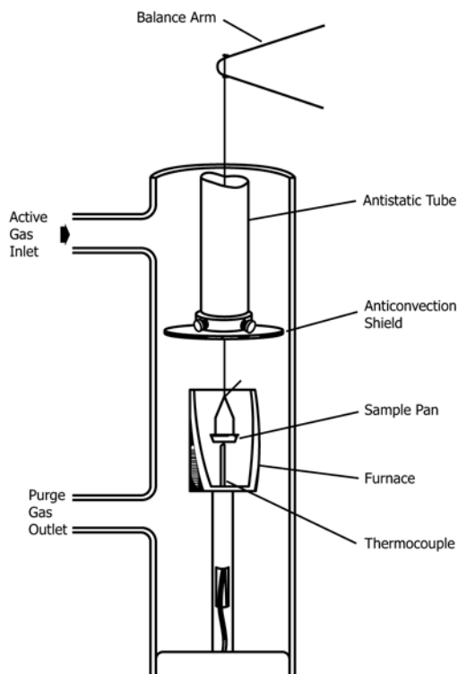
FIG. 4 Positioning of the Temperature Sensor (Thermocouple)
