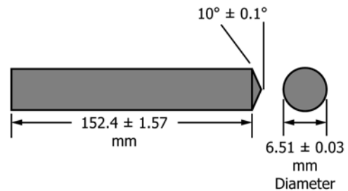
FIG. 1 Graphite Counter Electrode
