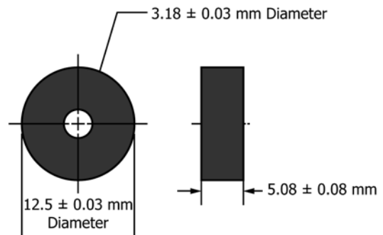
FIG. 2 Graphite Disc Electrode
