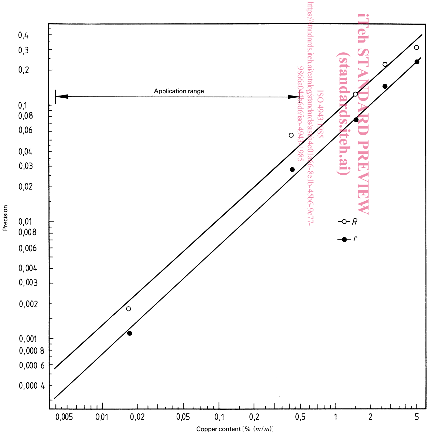
Figure — Relationship between copper content and repeatability, r , or reproducibility, R
