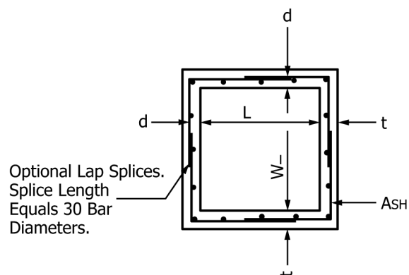
FIG. X1.2 Section AA
