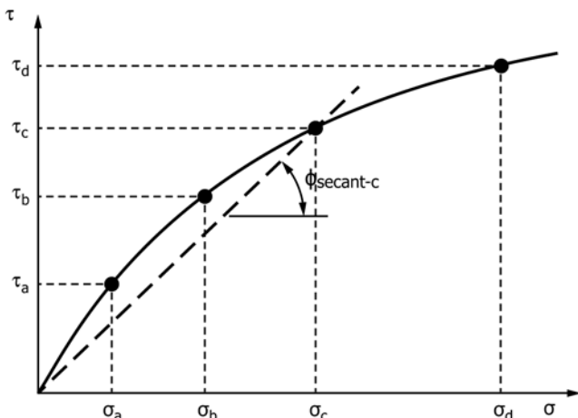
FIG. 8 Construction of a Curved Strength Envelope using Discrete Secant Friction Angles (USACOE (30))
