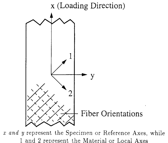
FIG. 2 Definition of Specimen and Material Axes
