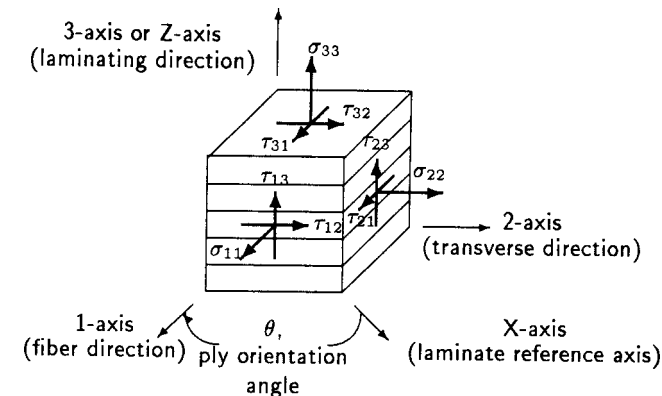
FIG. 1 Material Coordinate System
