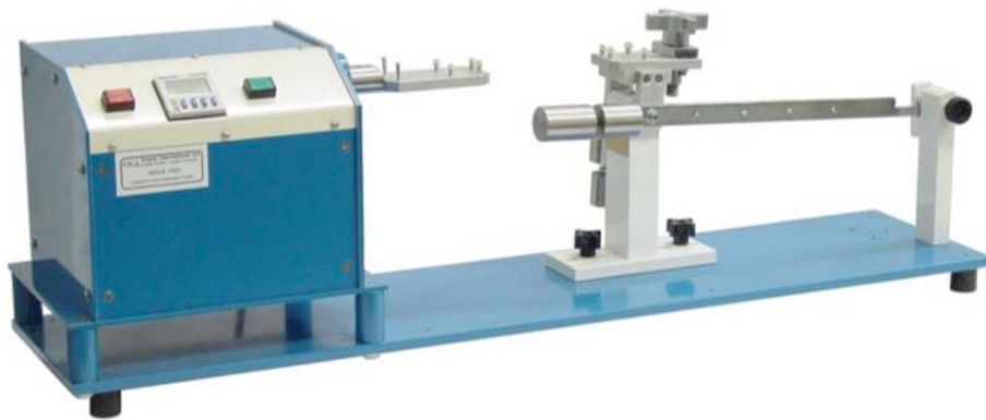
FIG. 1 Device for Preparing Twisted Pair Specimens, Motorized Unit
