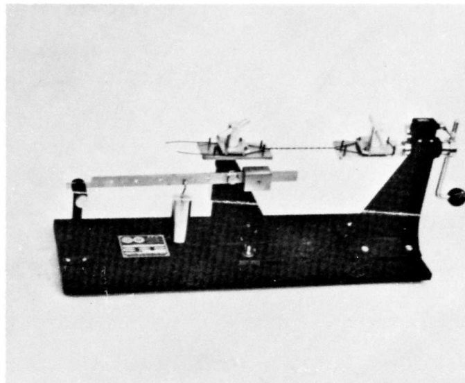
FIG. 2 Device for Preparing Twisted Pair Specimens, Hand-Operated Hand-operated Unit
