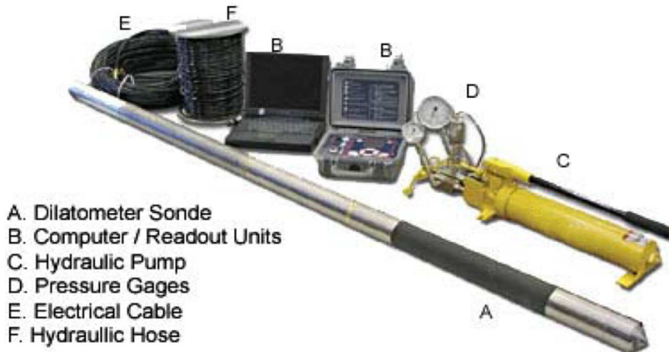
FIG. 34 Example of One Type of Volumetric Dilatometer Shown in Fig. 23.
