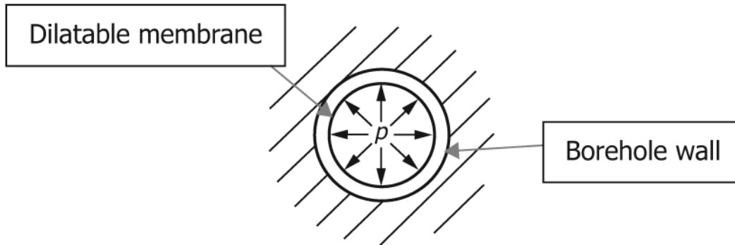
FIG. 52 Cross-Sections B-B 1 of the Borehole and Dilatable Membrane Portion of the Dilatometer in the Uninflated, r = 0 , Starting Position
