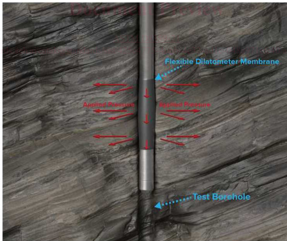
FIG. 1 General Depiction of a Flexible Dilatometer-Dilatometer, Deflated (a) and Inflated (b) in a Borehole
