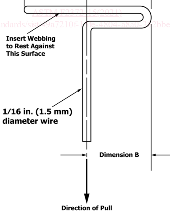
FIG. 2 Webbing Tension Pull Device
