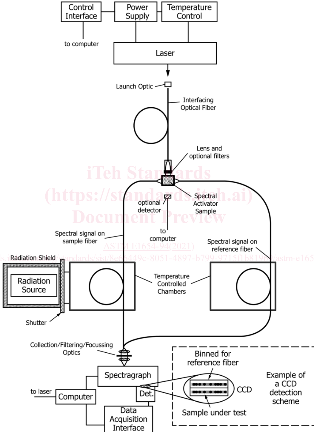
FIG. 1 Test Configuration
