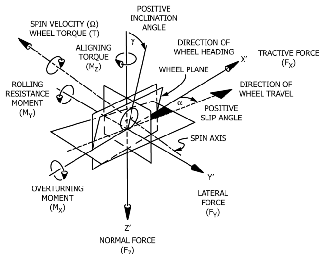
FIG. 1 Tire-Axis System
