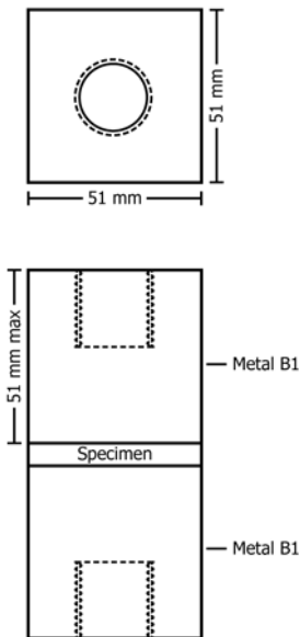
FIG. 1 Test Assembly for Bond Strength Test
