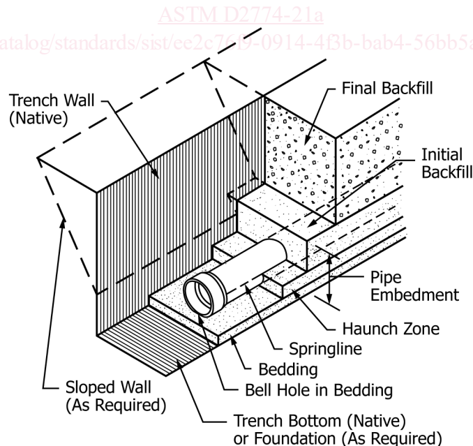
FIG. 1 Installation Terminology
