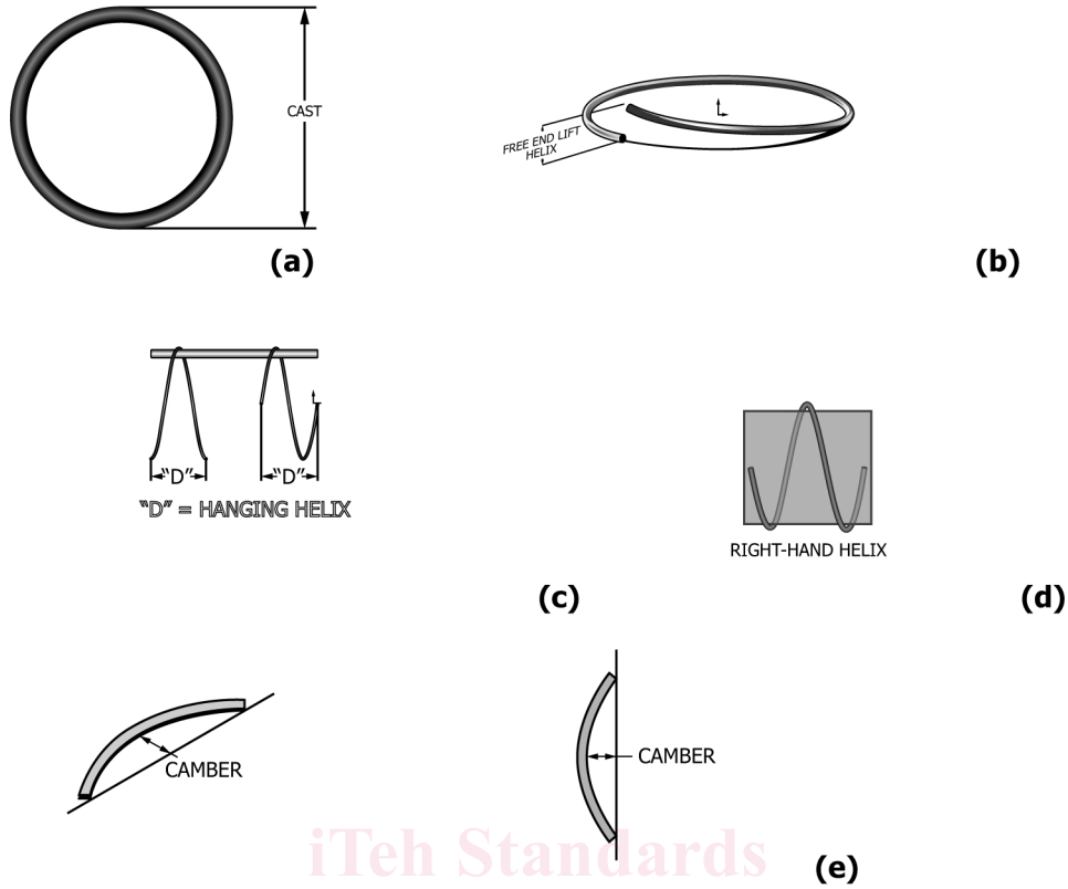
NOTE 1—(a) Definition of cast; (b) Definition of helix as measured by lift method; (c) Definition of helix as measured by hanging method; (d) Definition of helix direction; (e) Definition of camber.
