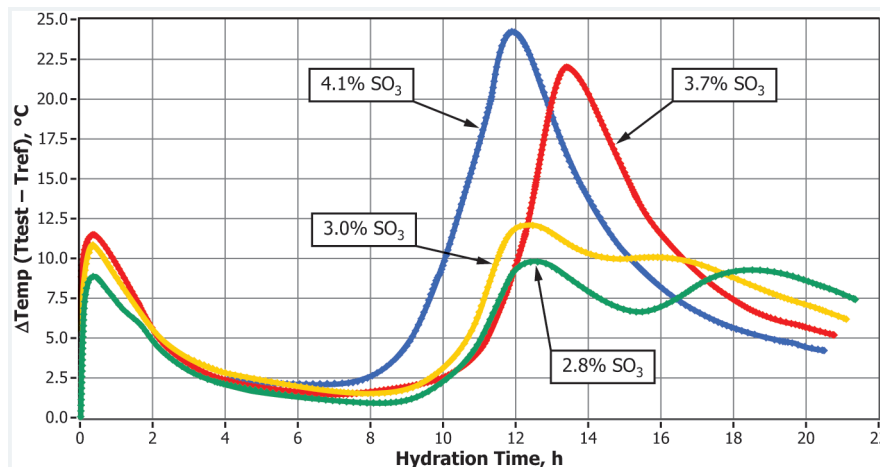
FIG. X1.1 The Effects of Incremental Cement SO 3 Content on Main Peak Response for a Mixture with 25% Class C Fly Ash Replacement and Water Reducing Admixture at 35 °C [95 °F] Initial Mixture and Test Temperatures, w/cm = 0.40
