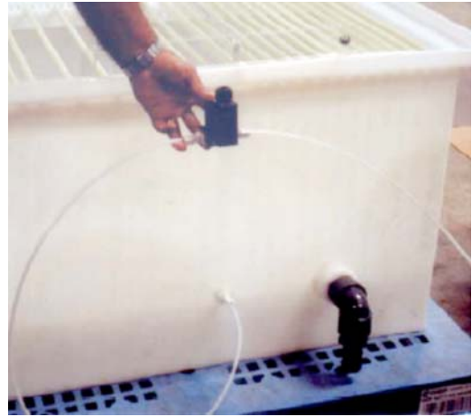
FIG. 12 Solenoid Valve with Tubing Connected
