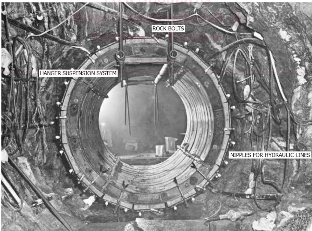
FIG. 6 Completed Setup of the Radial Jacking Test Reaction Frame and Extensometer Instrumentation Before Concrete Placement Around the Annular Space (1) Courtesy of US Bureau of Reclamation
