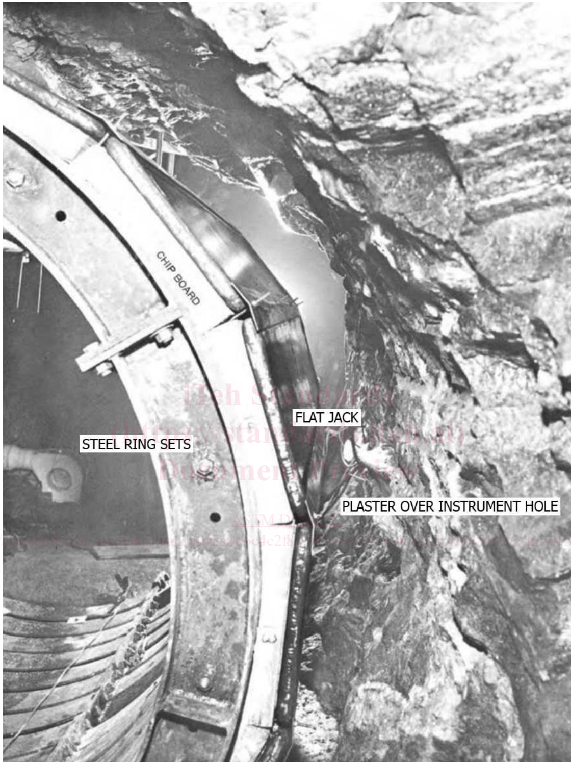
FIG. 7 Close-up of Reaction Frame Segments, Chipboard, Plaster Protection of Instrument Holes, and Flat Jacks Before Placing Concrete Between the Frame and Tunnel Wall (1)
