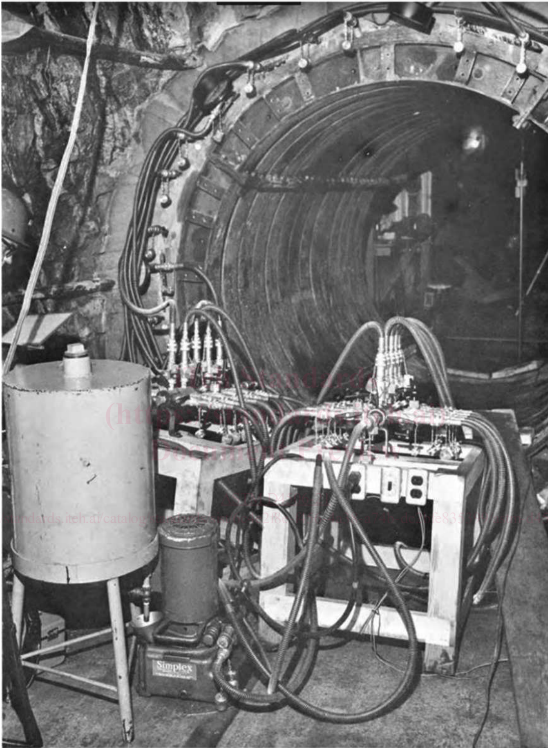
FIG. 8 View of Completed Radial Jacking Set Up with Loading Equipment and All Pressure Lines, Extensometers Cables, and Loading System Properly Connected and Secured (1) Courtesy of US Bureau of Reclamation
