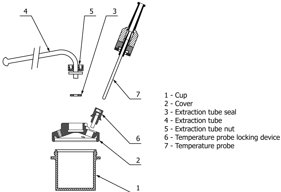
FIG. 3 Crucible with Temperature Probe
