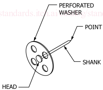
POWER-ACTUATED FASTENER
