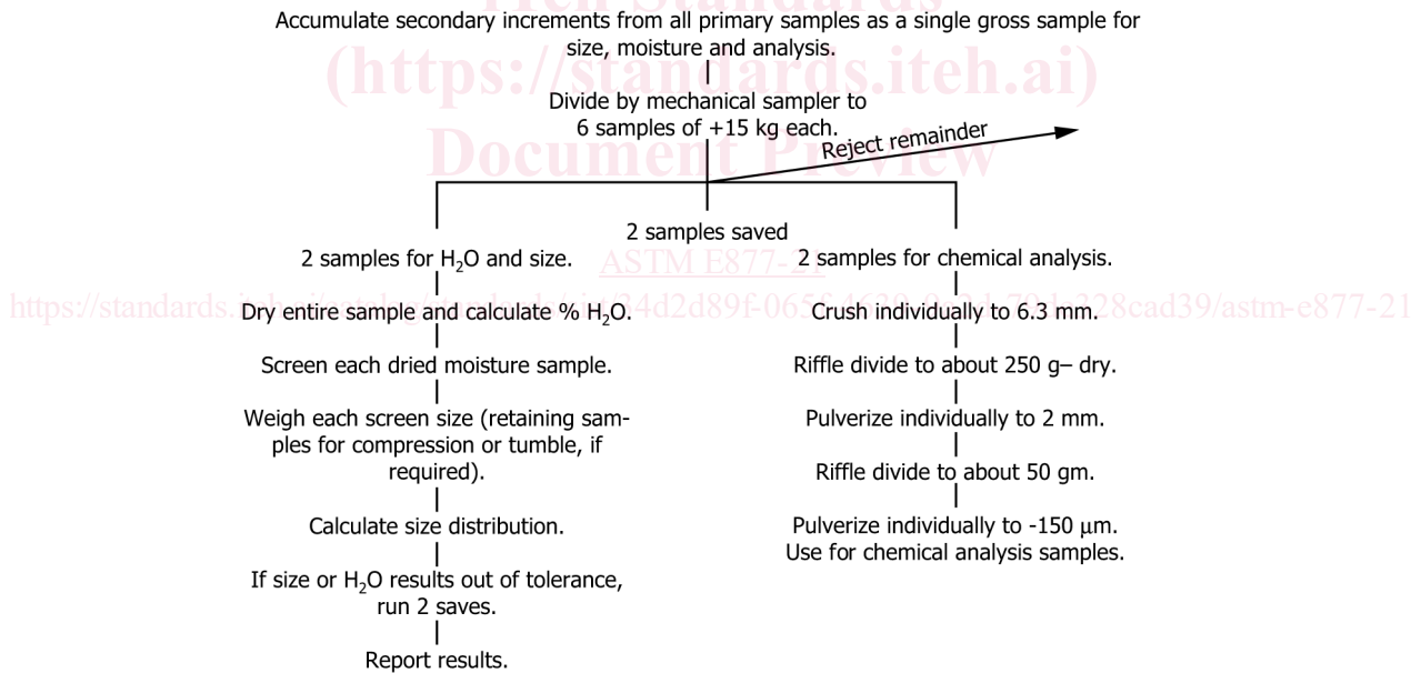
FIG. 3 Flowsheet Examples
