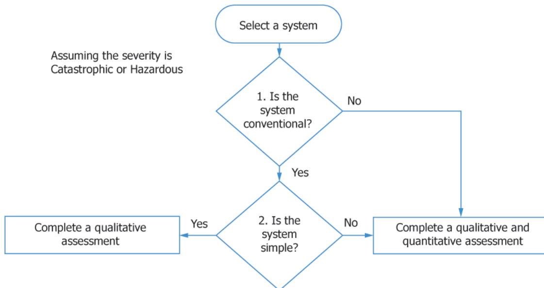
FIG. X2.1 Process Overview
