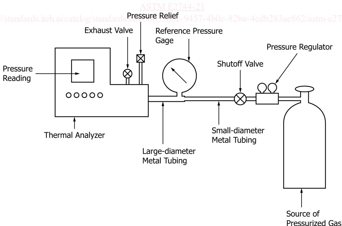
FIG. 1 Schematic Diagram of Apparatus
