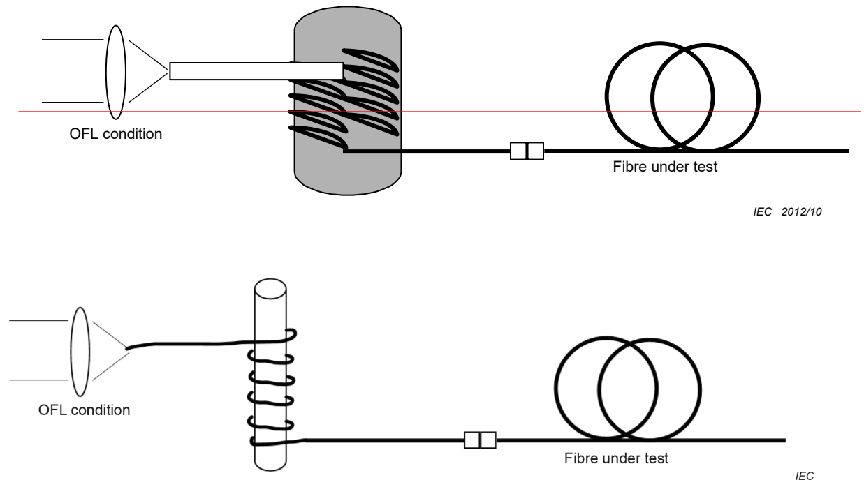
Figure 1 – Mandrel wrapped mode filter
