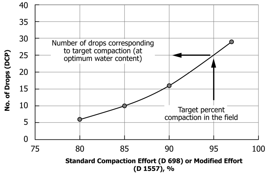
FIG. 5 Calibration of No. of Drops with Soil Percent Compaction
