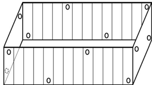
FIG. 1 (a) Immersion Bath With Permanently Attached AE Sensors on Exterior (Circles)
