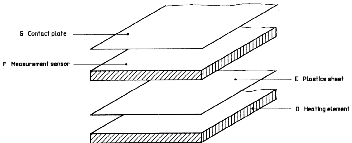
Figure 2 — Details of heating body
