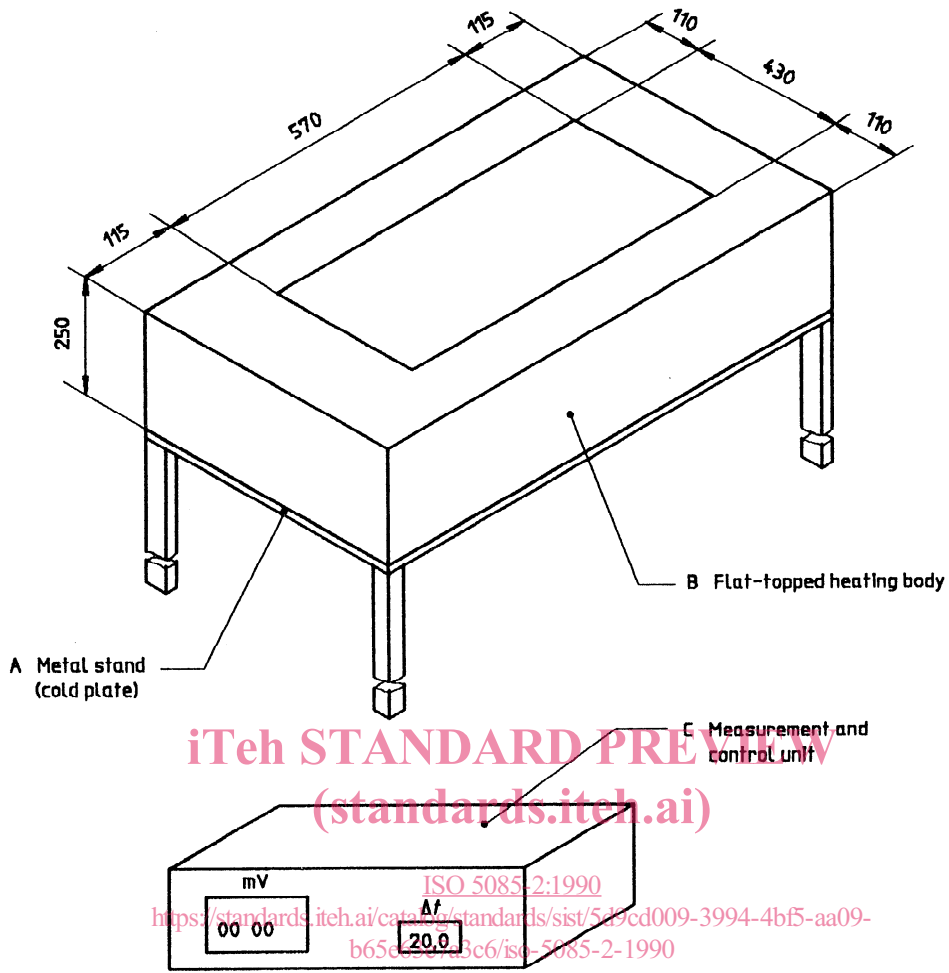
Figure 1 — Flat-topped heating body
