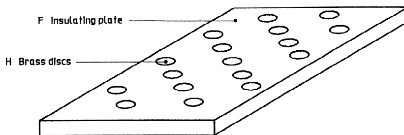
Figure 3 — Details of measurement sensor
